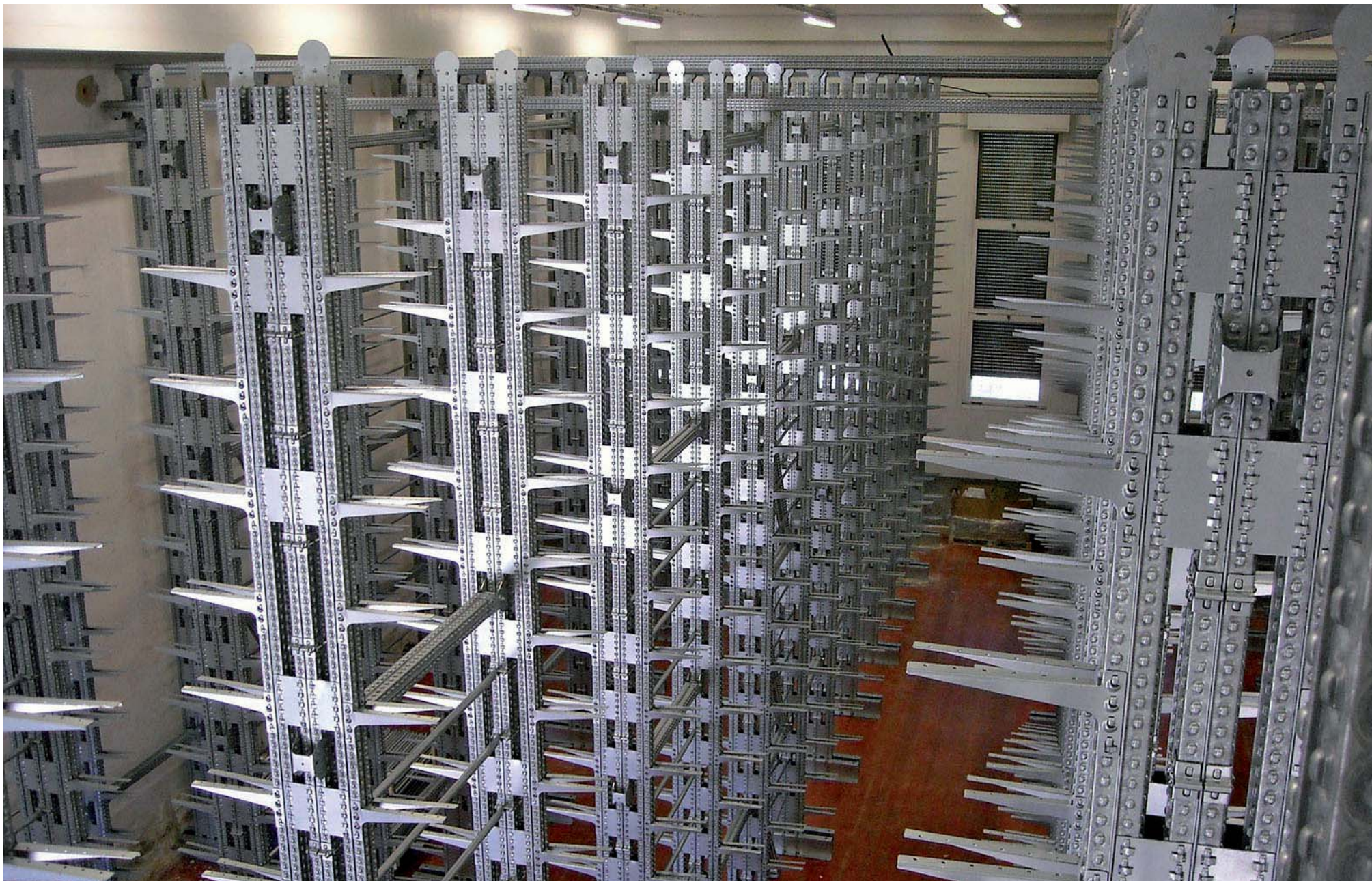
METALSISTEM Seismic Racking Structure designed for a Dairy Factory - High Density Storage of Parmesan Cheese <October 2012>
