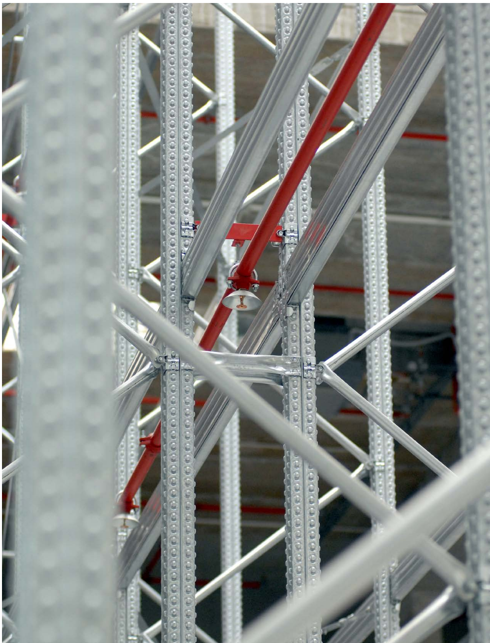
Super 4-5-6 Pallet racking installation. <September 2013>
