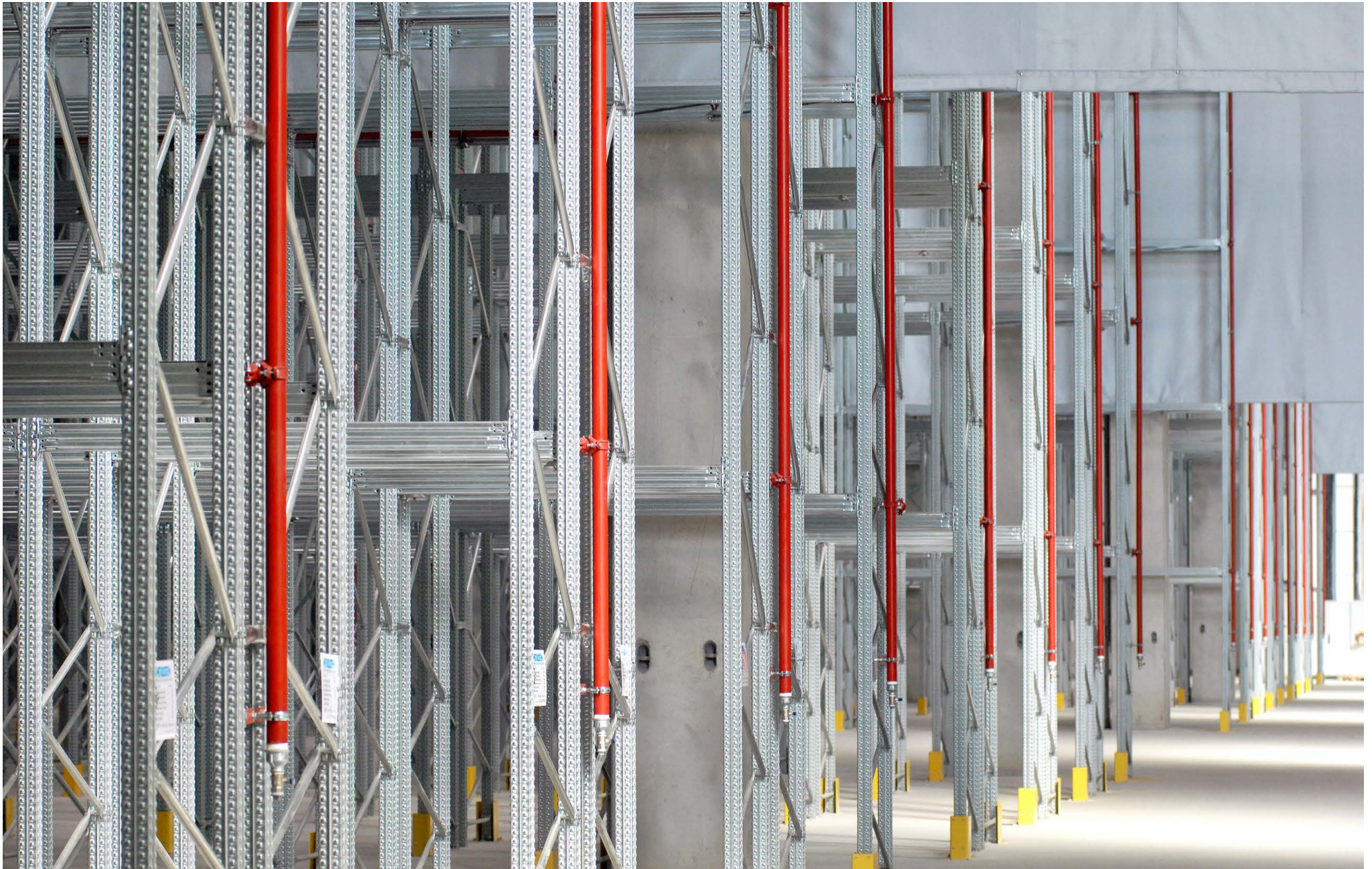
Super 4-5-6 Pallet racking installation. <September 2013>
