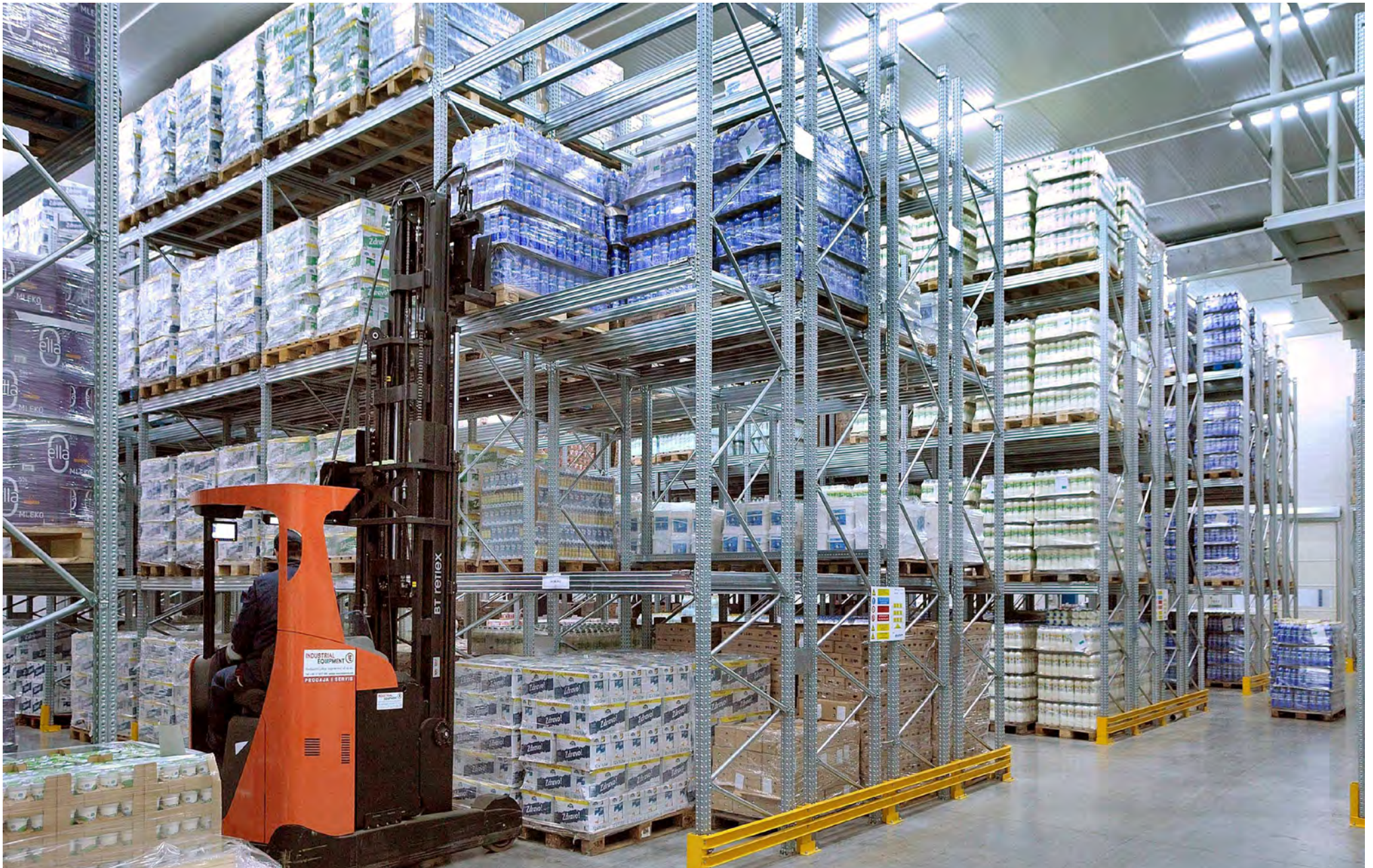
Dairy plant reference installation - Super 4-5-6 Pallet Racking & Drive-In <May 2014>
