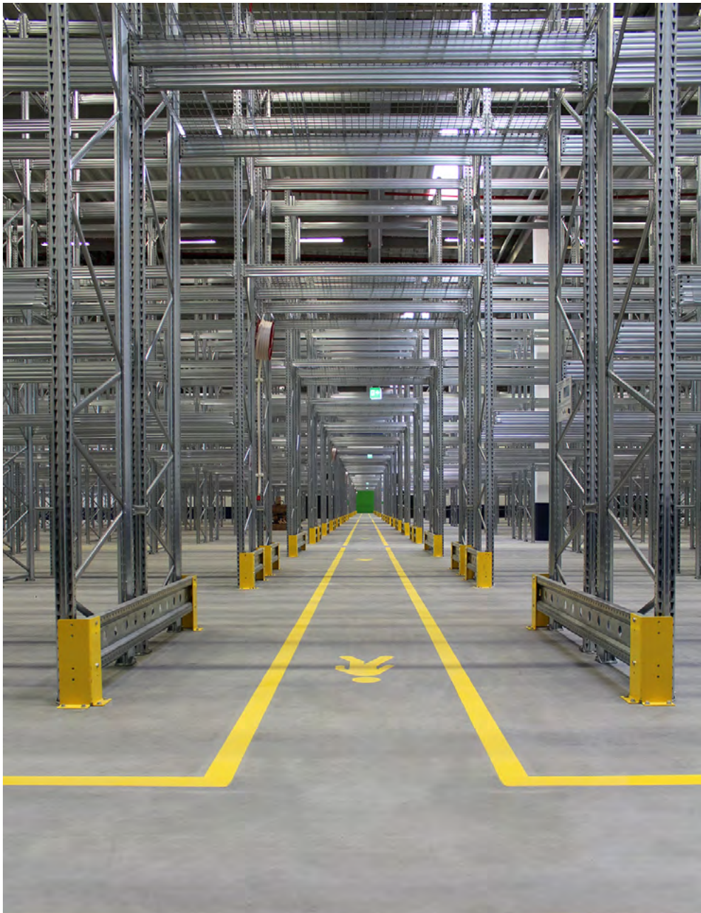
SUPERBUILD - Pallet Racking Reference Installation - Pharmaceutical Products.
